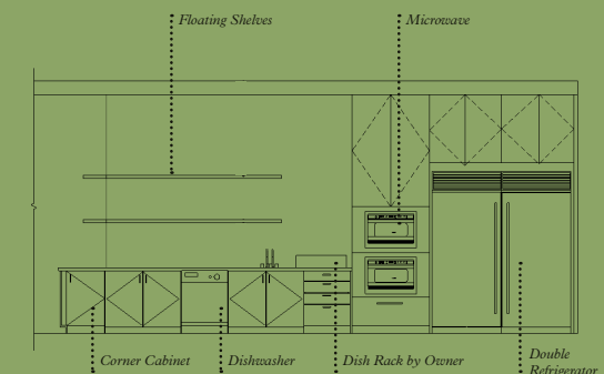
Breakroom Pantry Elevation
