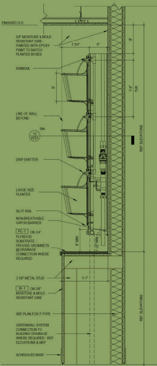
Green Wall Section Detail
