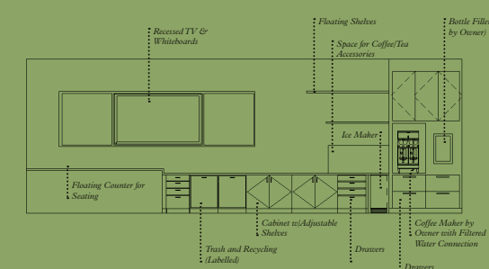
Breakroom Pantry Elevation
